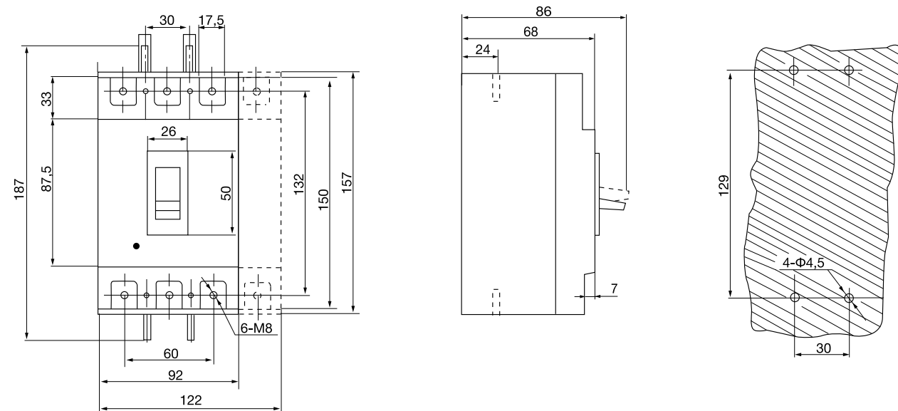
BA88-31
