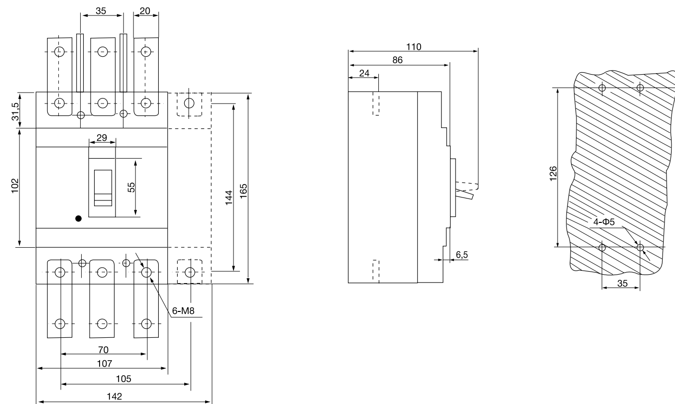
BA88-35
