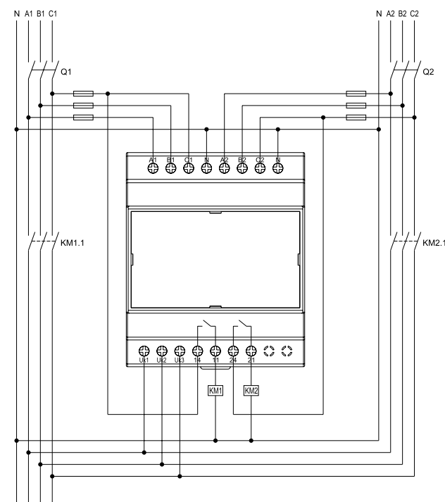
ETS-2ZC
